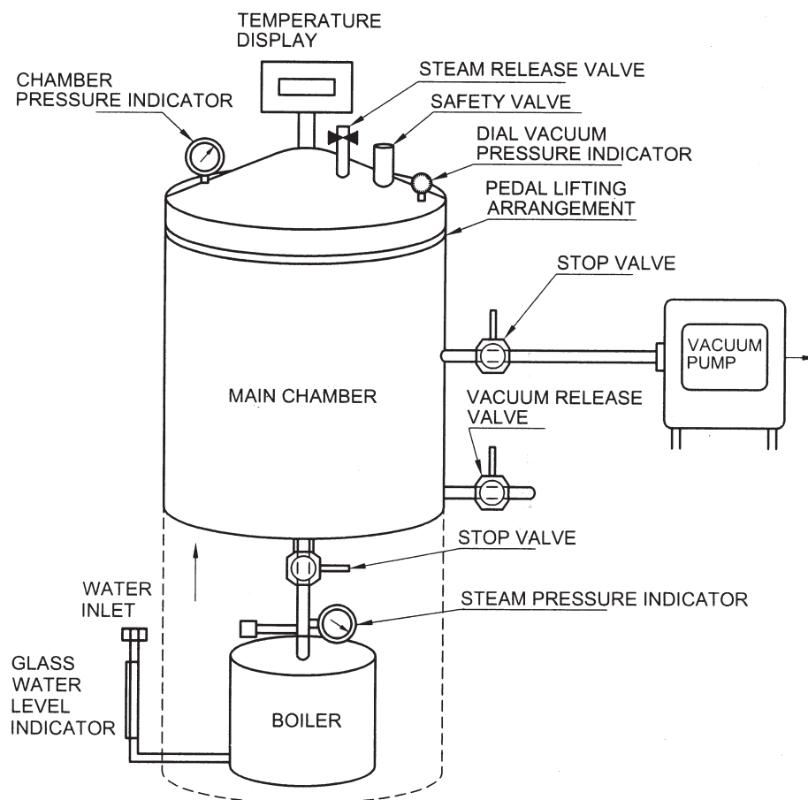
FIG. 1 VACUUM STEAM PRESSURE TEST (VPT) APPARATUS
